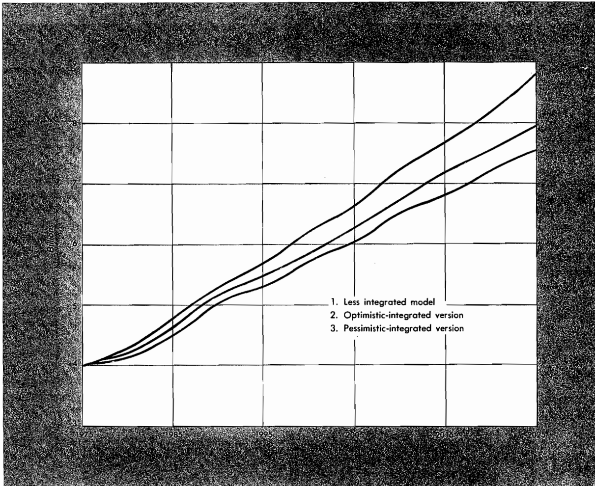
Figure 31-13. Global population projections for three versions of the World Intergrated Model.
