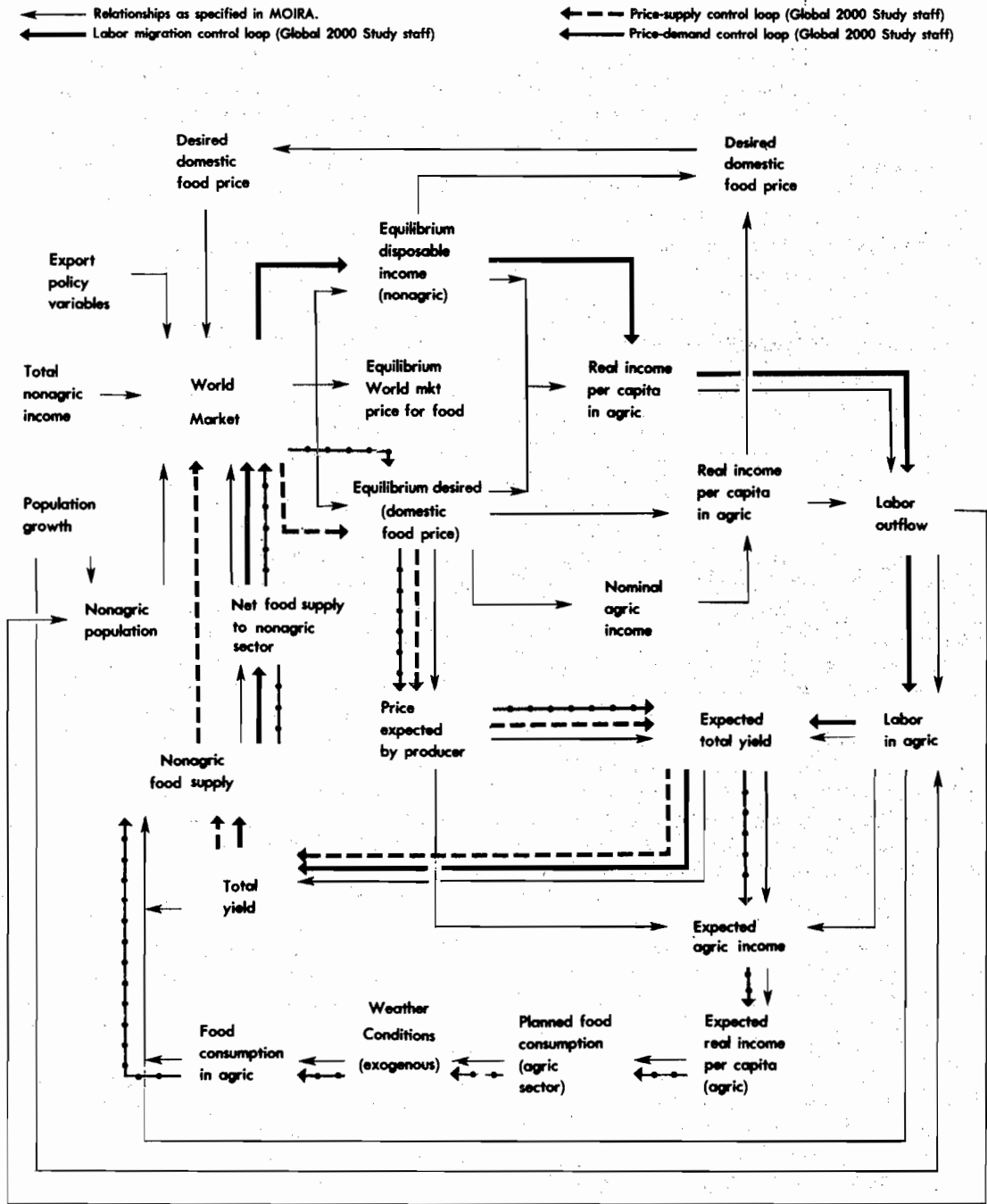
Figure 27-1. Channels of causal influence and major feedback controls in MOIRA. (Hans Linnemann, MOIRA: A Model of International Relations in Agriculture, forthcoming)
