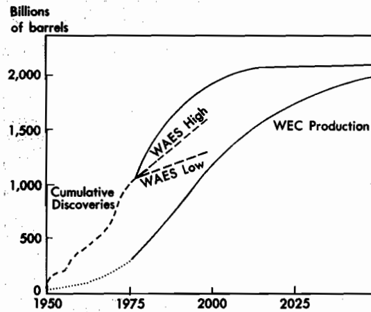
Figure 10-4. Cumulative world discovery and production of oil.
